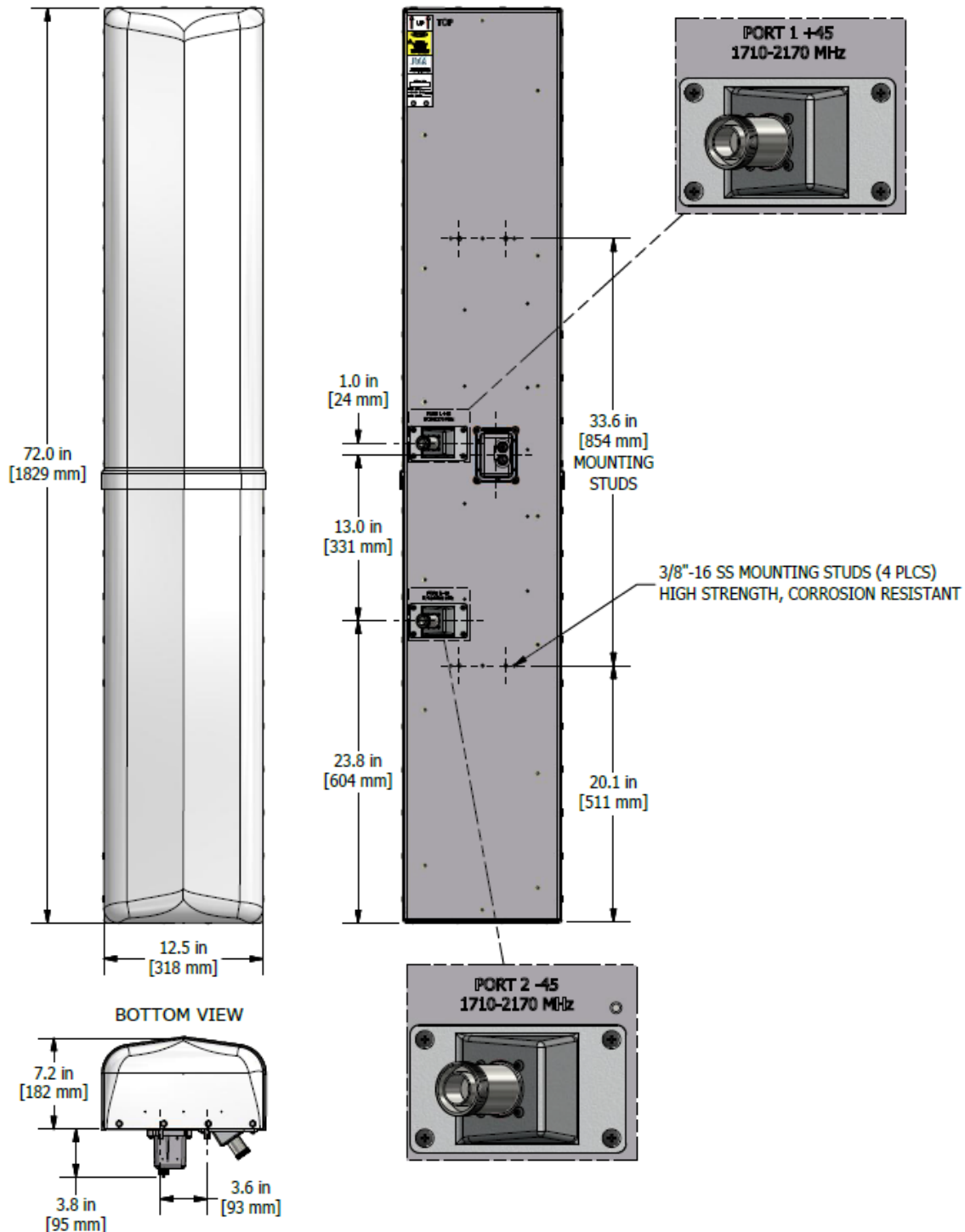
FRONT VIEW
