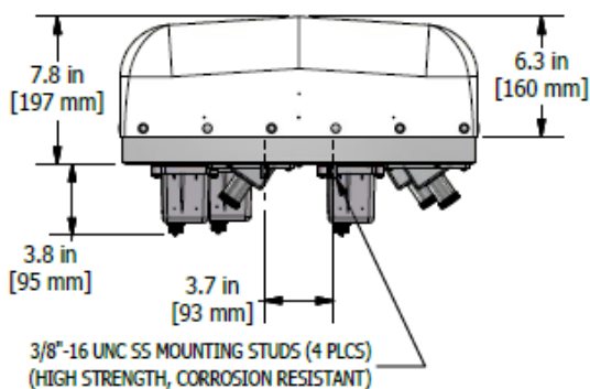
BOTTOM VIEW
